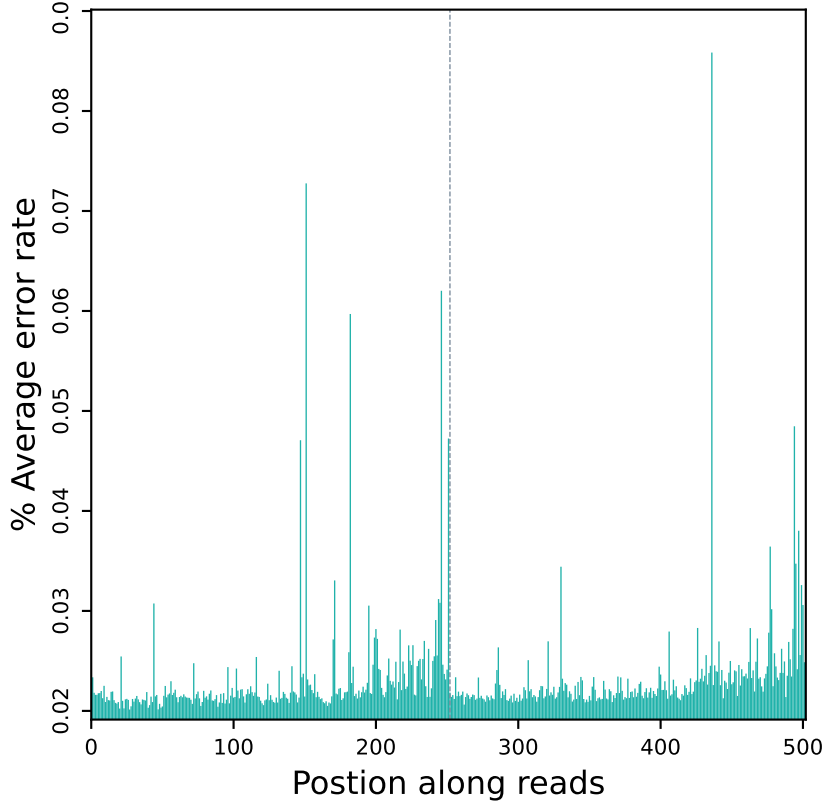
Error rate distribution along reads (R10729)
